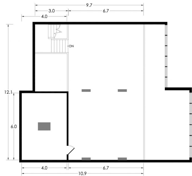
MEZZANINE LEVEL
